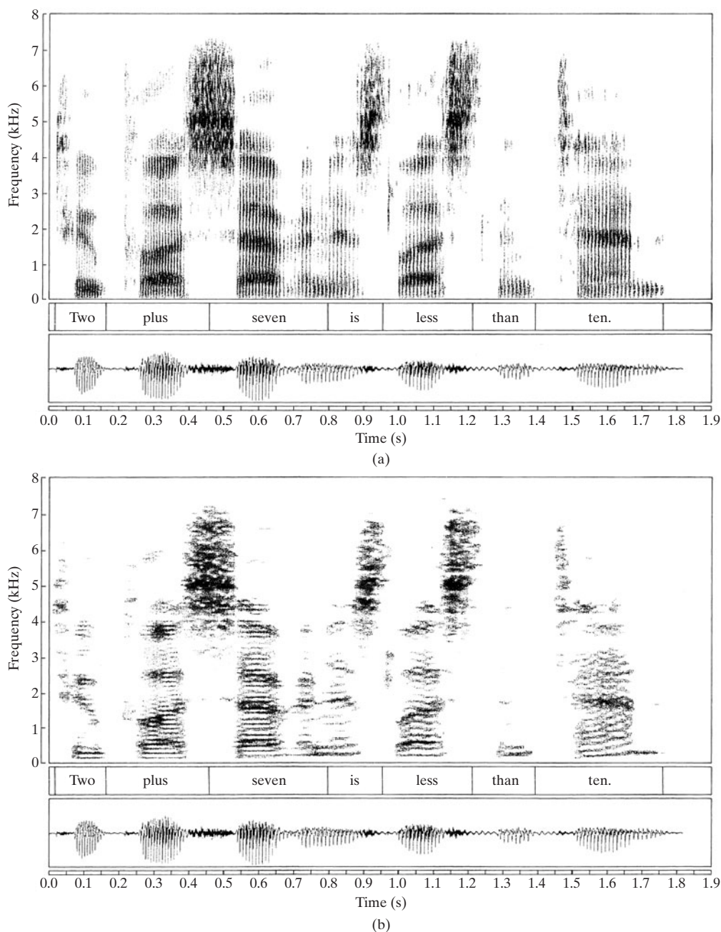
Figure 10.22 (a) Wideband spectrogram of waveform of Figure 10.21. (b) Narrowband spectrogram.
