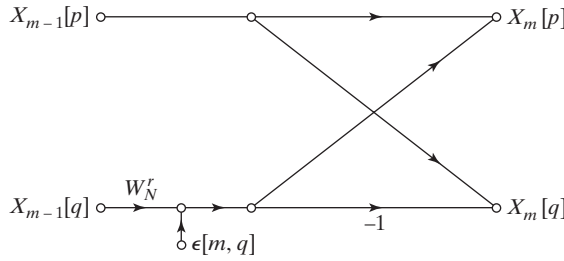
Figure 9.36 Linear-noise model for fixed-point round-off noise in a decimation-in-time butterfly computation.
