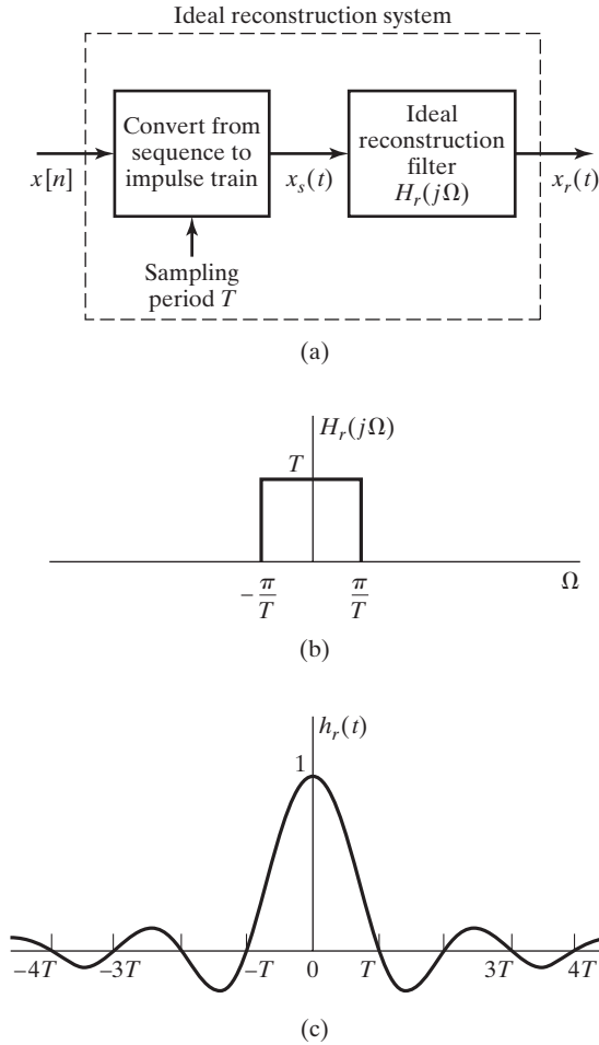
Figure 4.7 (a) Block diagram of an ideal bandlimited signal reconstruction system. (b) Frequency response of an ideal reconstruction filter. (c) Impulse response of an ideal reconstruction filter.
