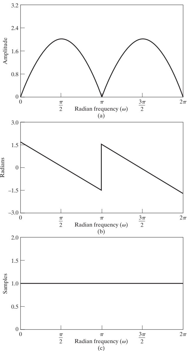
Figure 5.36 Frequency response of type III system of Example 5.17. (a) Magnitude. (b) Phase. (c) Group delay.
