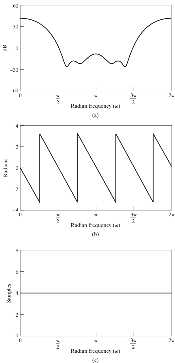
Figure 5.40 Frequency response of cascade of maximum-phase and minimum-phase systems, yielding a linear-phase system. (a) Log magnitude. (b) Phase (principal value). (c) Group delay.
