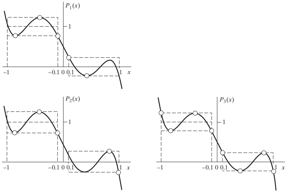
Figure 7.43 5 th -order polynomials for Example 7.8. Alternation points are indicated by ○.
