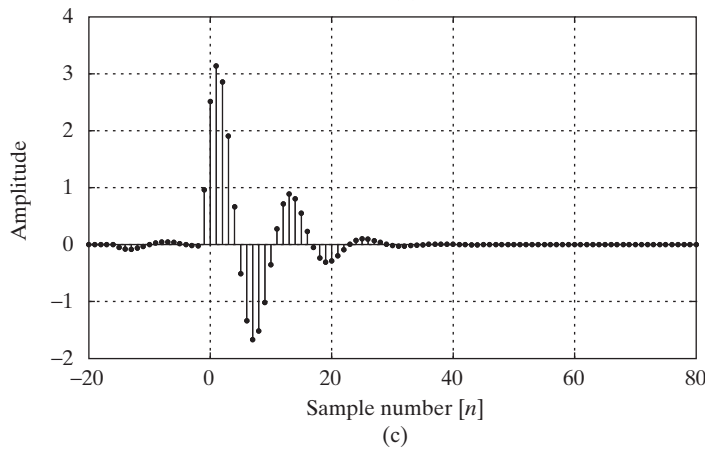
Figure 13.17 Lowpass frequency-invariant linear filtering in the system of Figure 13.15. (a) Real parts of the Fourier transforms of the input (solid line) and output (dashed line) of the lowpass system with N_1 = 14 and N_2 = 14 in Figure 13.16(a). (b) Imaginary parts of the input (solid line) and output (dashed line). (c) Output sequence y[n] for the input of Figure 13.10(c).
