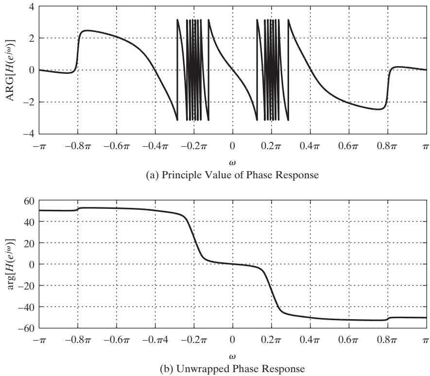
Figure 5.3 Phase response functions for system in the example of Section 5.1.2; (a) Principal value phase, \text{ARG}[H(e^{j\omega})] , (b) Continuous phase \arg[H(e^{j\omega})] .
