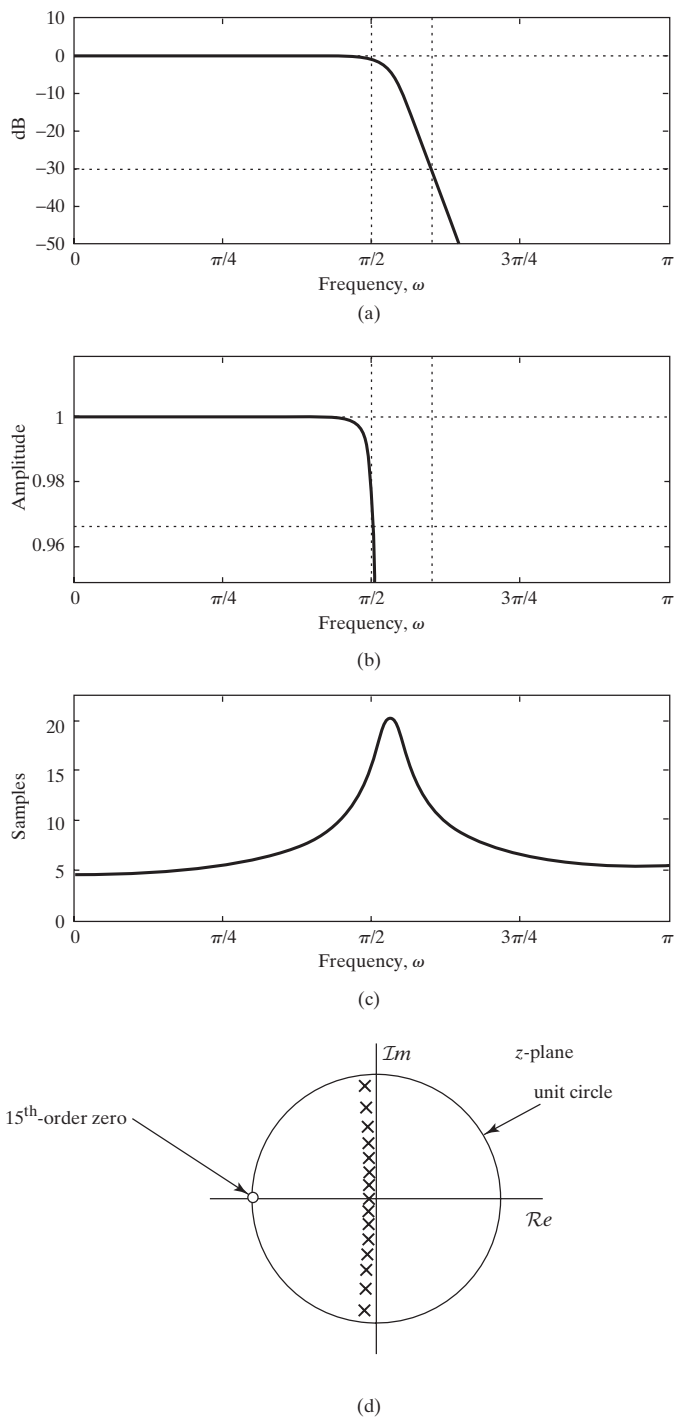
Figure 7.12 Butterworth filter, 15 th -order.
