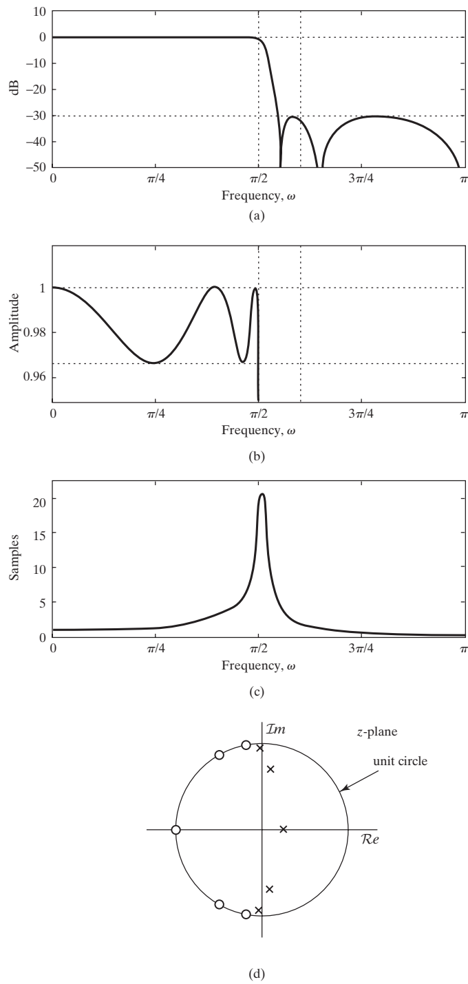
Figure 7.15 Elliptic filter, 5 th -order, exceeds design specifications.
