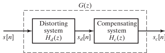
Figure 5.22 Illustration of distortion compensation by linear filtering.
