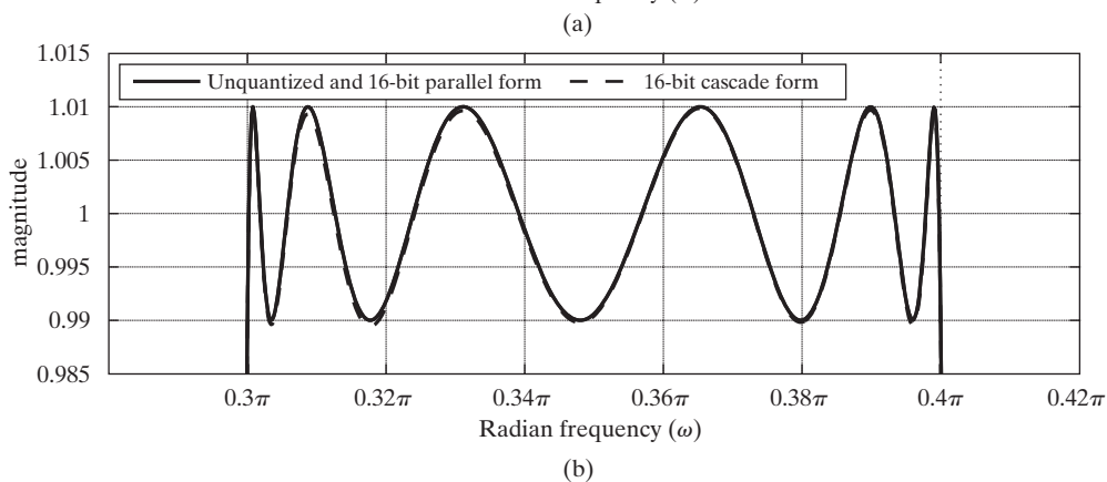
Figure 6.47 IIR coefficient quantization example. (a) Log magnitude for unquantized elliptic bandpass filter. (b) Magnitude in passband for unquantized (solid line) and 16-bit quantized cascade form (dashed line).
