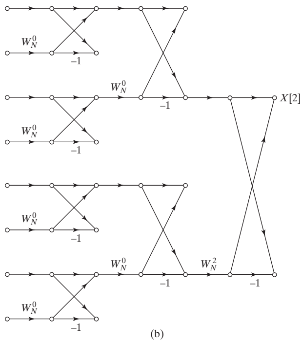
Figure 9.37 (a) Butterflies that affect X[0] ; (b) butterflies that affect X[2] .
