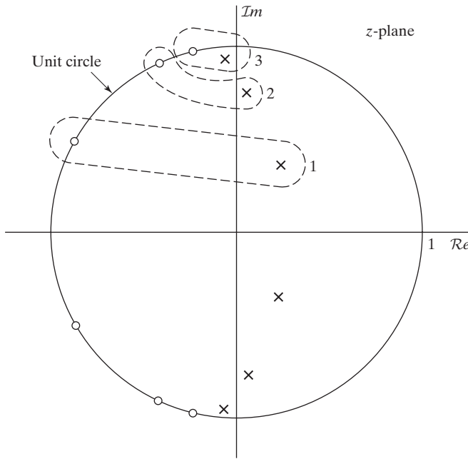
Figure 6.65 Pole-zero plot for 6 th -order system of Figure 6.64, showing pairing of poles and zeros.
