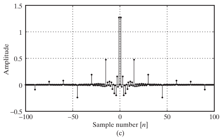
Figure 13.12 The sequences: (a) c_v[n] , (b) c_p[n] , and (c) c_x[n] .
