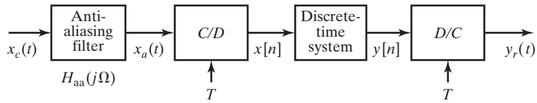
Figure 4.48 Use of prefiltering to avoid aliasing.
