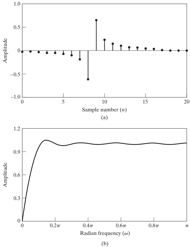
Figure 12.8 (a) Impulse response and (b) magnitude response of an FIR Hilbert transformer designed using the Kaiser window. ( M = 17 and \beta = 2.44 .)
