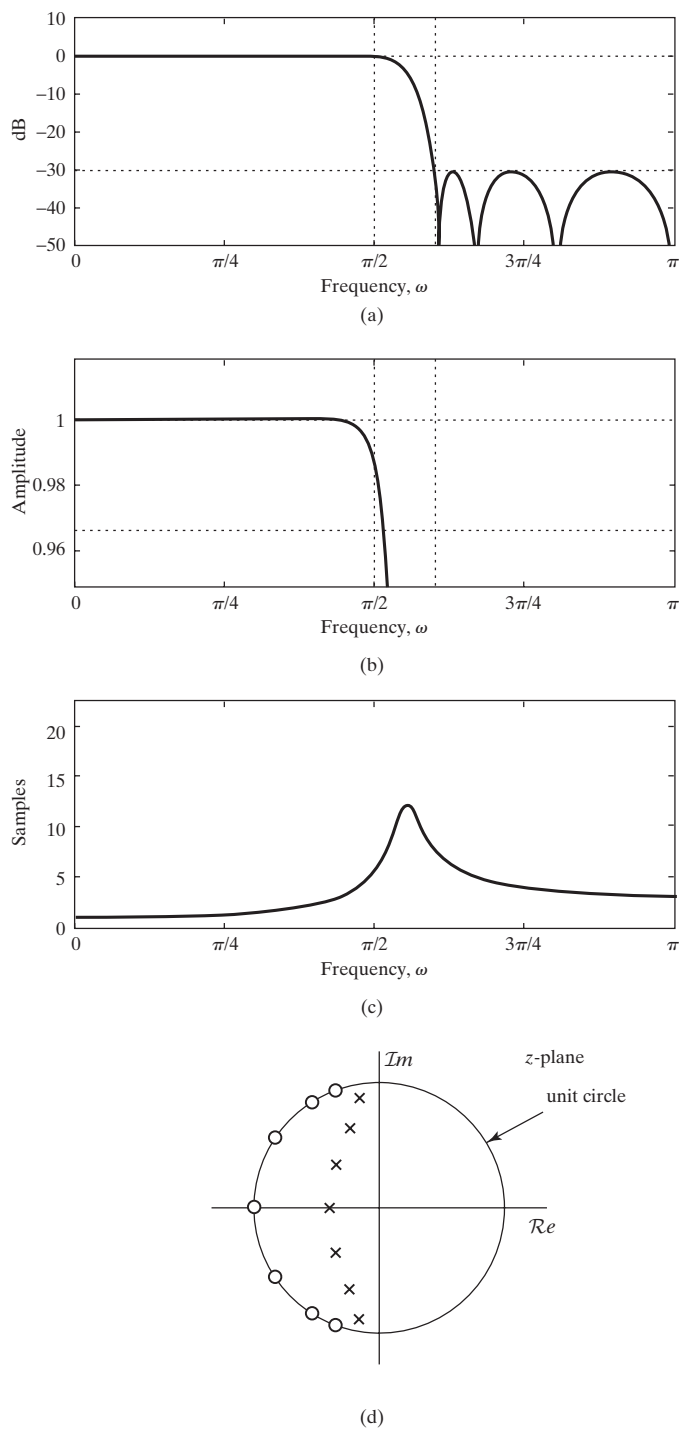
Figure 7.14 Chebyshev Type II filter, 7 th -order.
