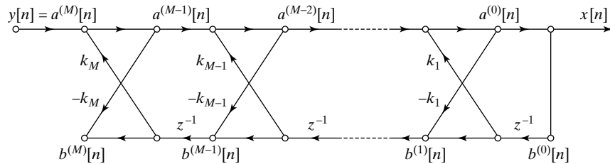
Figure 6.42 All-pole lattice system.
