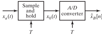
Figure 4.51 Physical configuration for A/D conversion.
