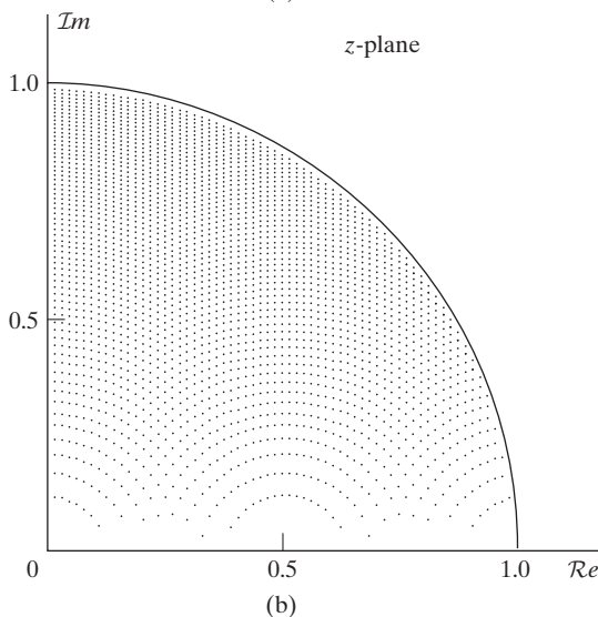
Figure 6.50 Pole-locations for the 2 nd -order IIR direct form system of Figure 6.49. (a) Four-bit quantization of coefficients. (b) Seven-bit quantization.
