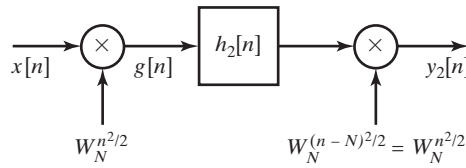
Figure 9.33 Block diagram of chirp transform system for obtaining DFT samples.
