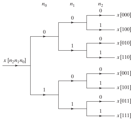
Figure 9.14 Tree diagram depicting bit-reversed sorting.
