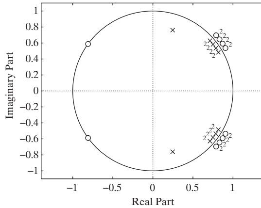
Figure 5.2 Pole-zero plot for the filter in the example of Section 5.1.2. (The number 2 indicates double-order poles and zeroes.)
