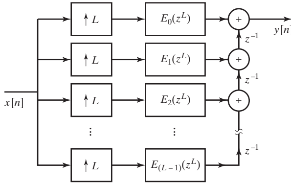
Figure 4.42 Implementation of interpolation filter using polyphase decomposition.
