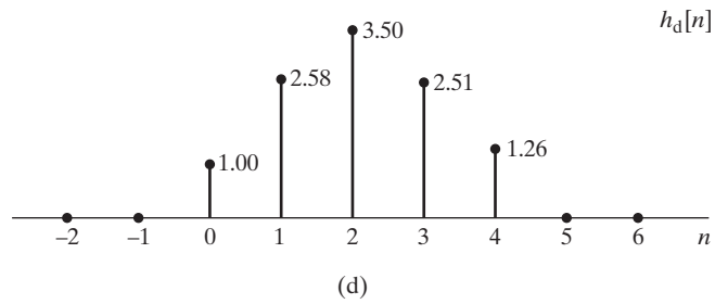
Figure 5.28 Sequences corresponding to the pole-zero plots of Figure 5.27.
