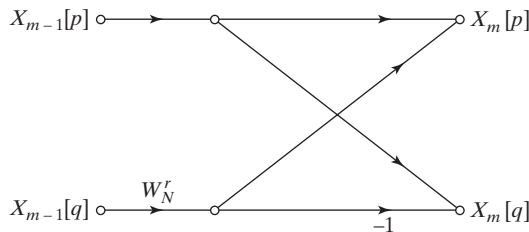
Figure 9.35 Butterfly computation for decimation-in-time.
