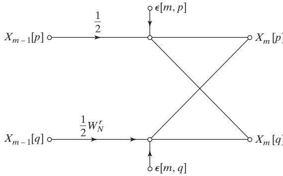
Figure 9.38 Butterfly showing scaling multipliers and associated fixed-point round-off noise.
