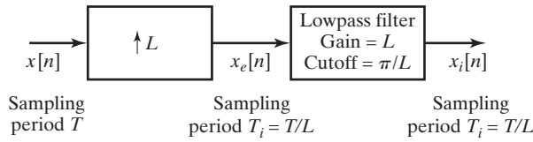
Figure 4.23 General system for sampling rate increase by L .
