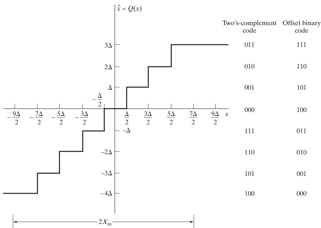
Figure 4.54 Typical quantizer for A/D conversion.
