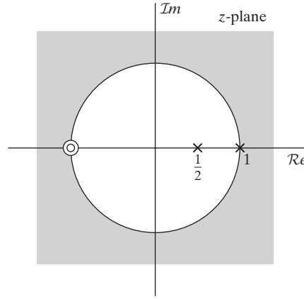
Figure 3.11 Pole-zero plot for the z -transform in Example 3.10.
