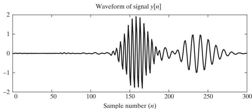
Figure 5.6 Output signal for the example of Section 5.1.2.
